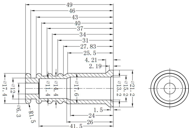
(Schematic Diagram)
